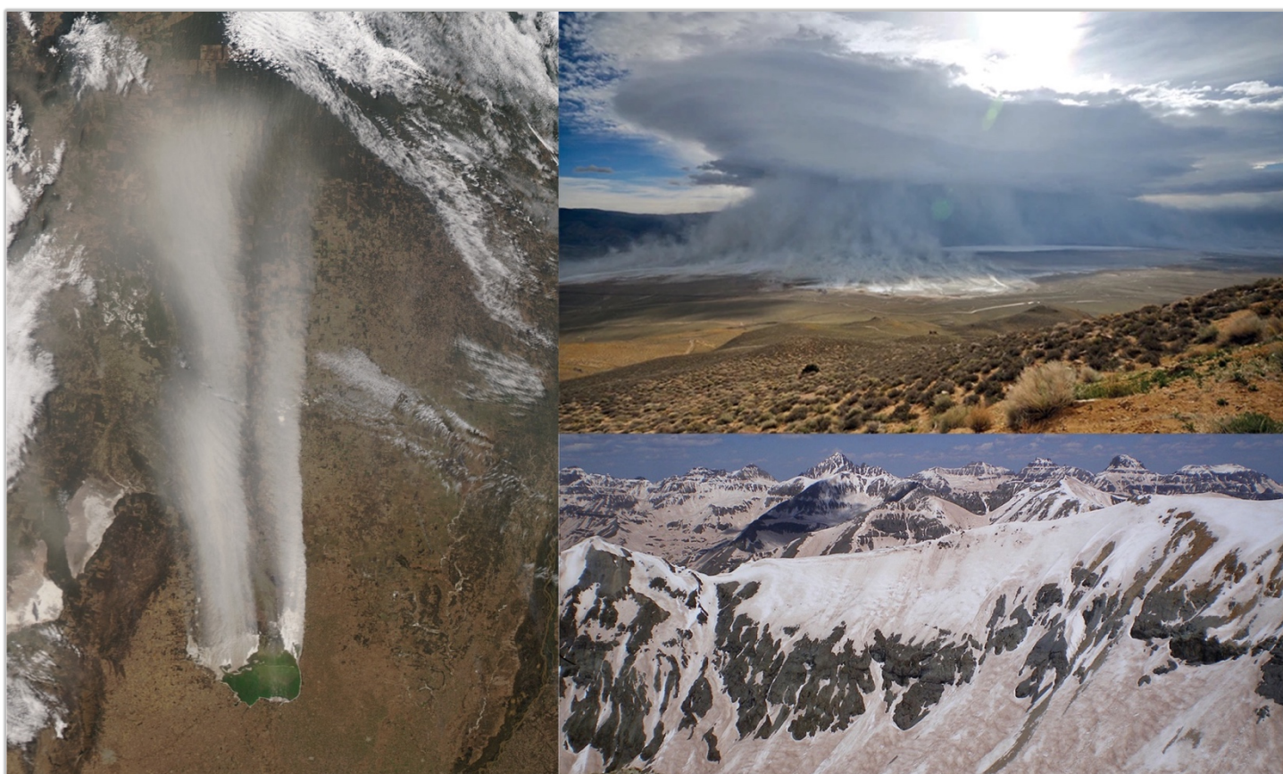
Figure 8. Dust from drying saline lakes. Left: Mar Chiquita, Argentina (NASA, Jeff Schmaltz). Upper right: Owens Lake, California (Brian Russell). Lower right: dust darkens snowpack in the Rockies causing early melt (NASA).
